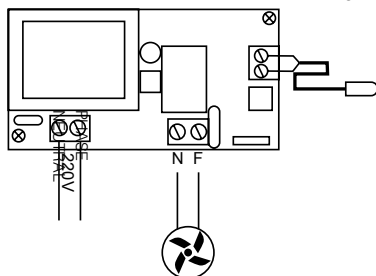
Switchboard wiring diagram
